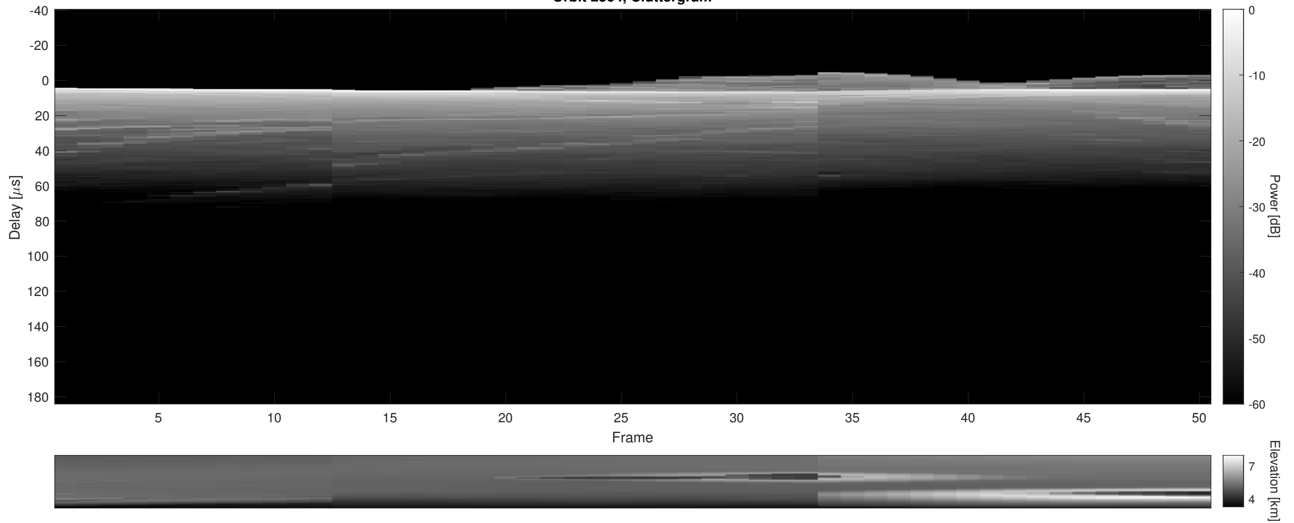
Orbit 2364, Cluttergram
