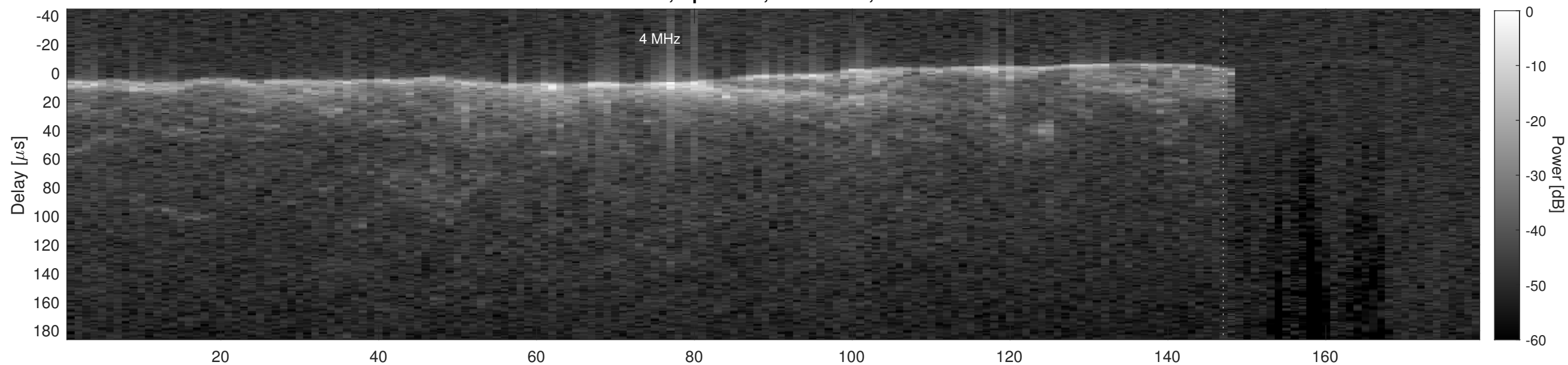
Orbit 2366, Cluttergram
