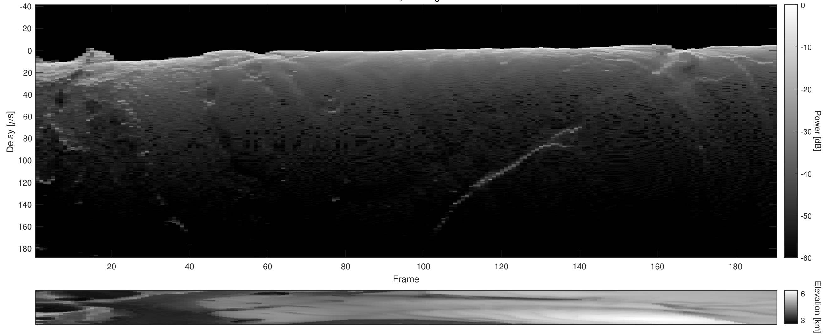
Orbit 2369, Cluttergram
