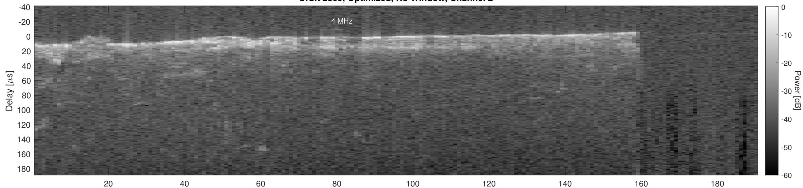
Orbit 2369, Cluttergram
