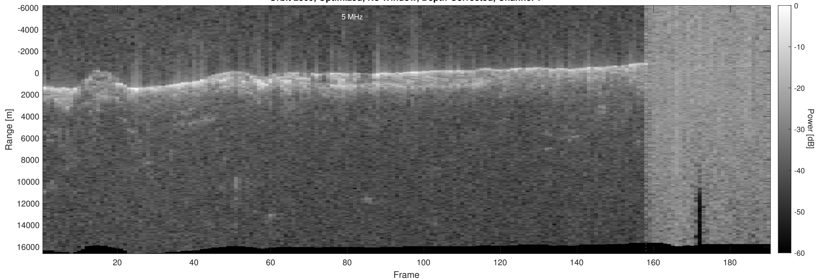
Orbit 2369, Optimized, No Window, Depth-Corrected, Channel 2
