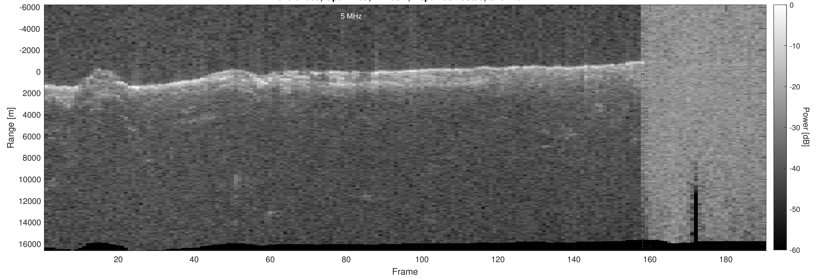
Orbit 2369, Optimized, Window, Depth-Corrected, Channel 2
