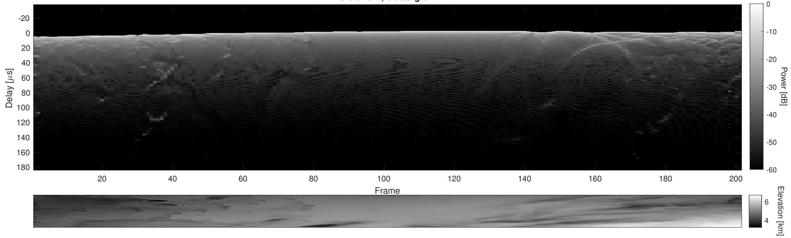
Orbit 2372, Cluttergram
