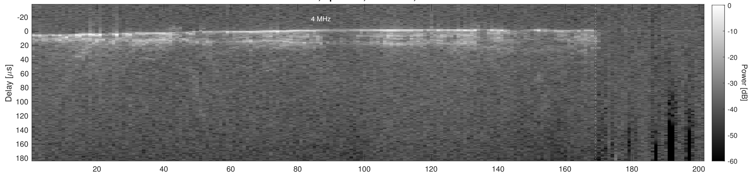
Orbit 2372, Cluttergram
