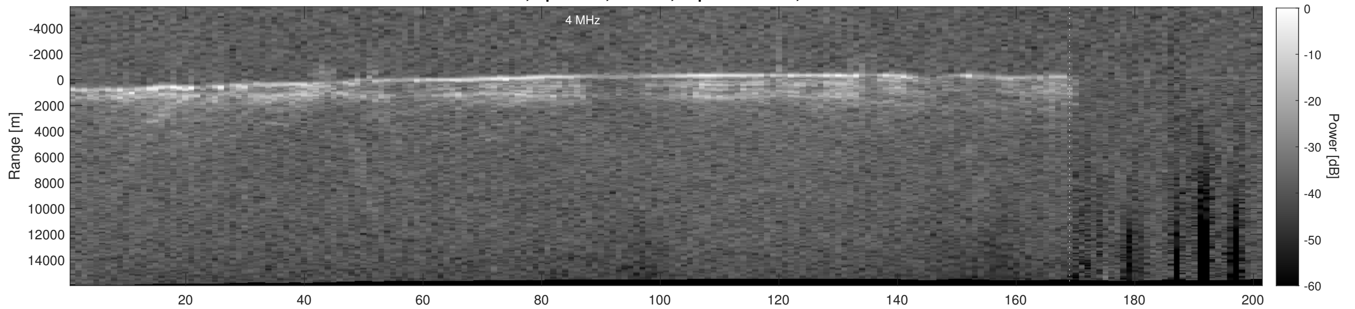
Orbit 2372, Depth-Corrected Cluttergram
