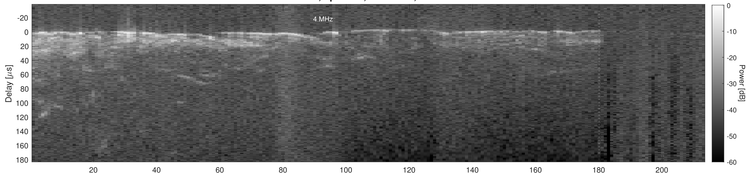
Orbit 2376, Cluttergram
