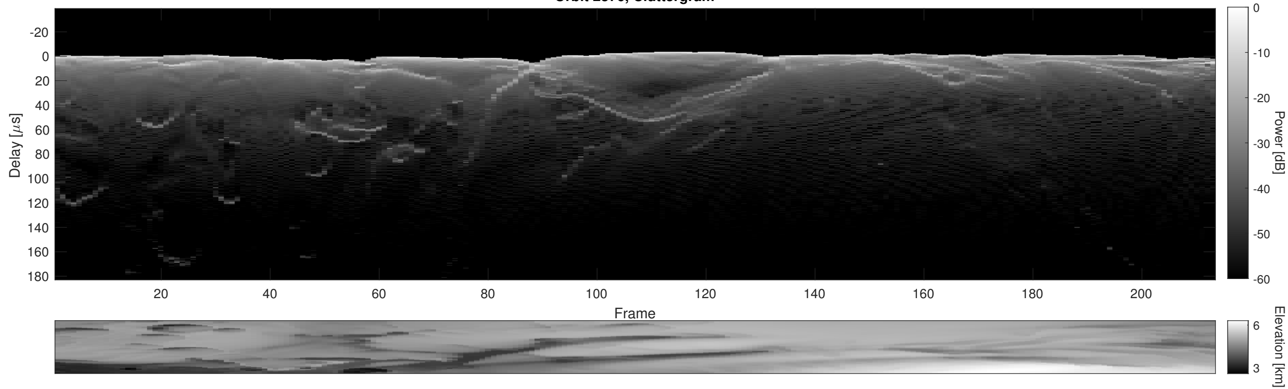
Orbit 2376, Cluttergram
