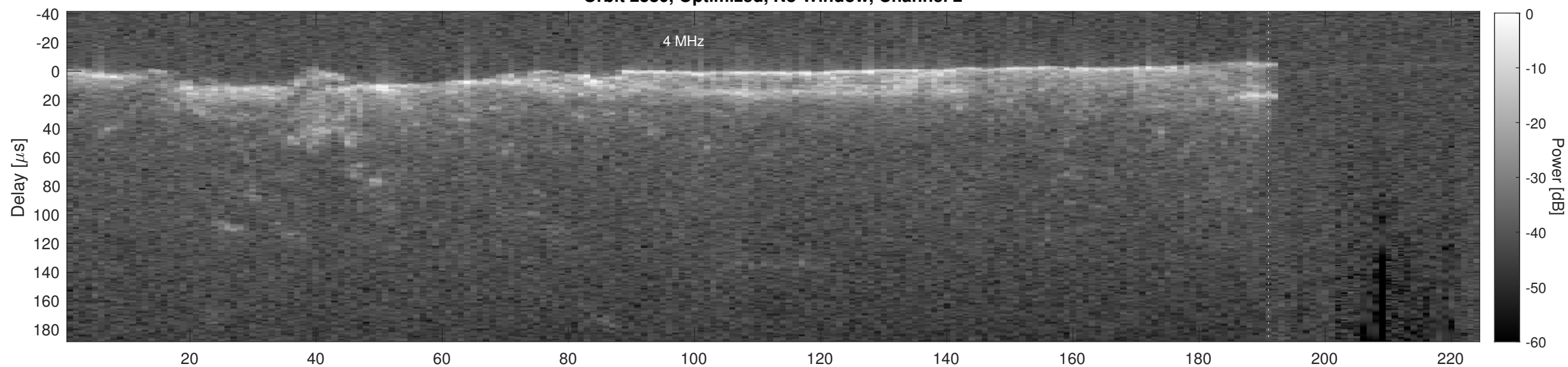
Orbit 2380, Cluttergram
