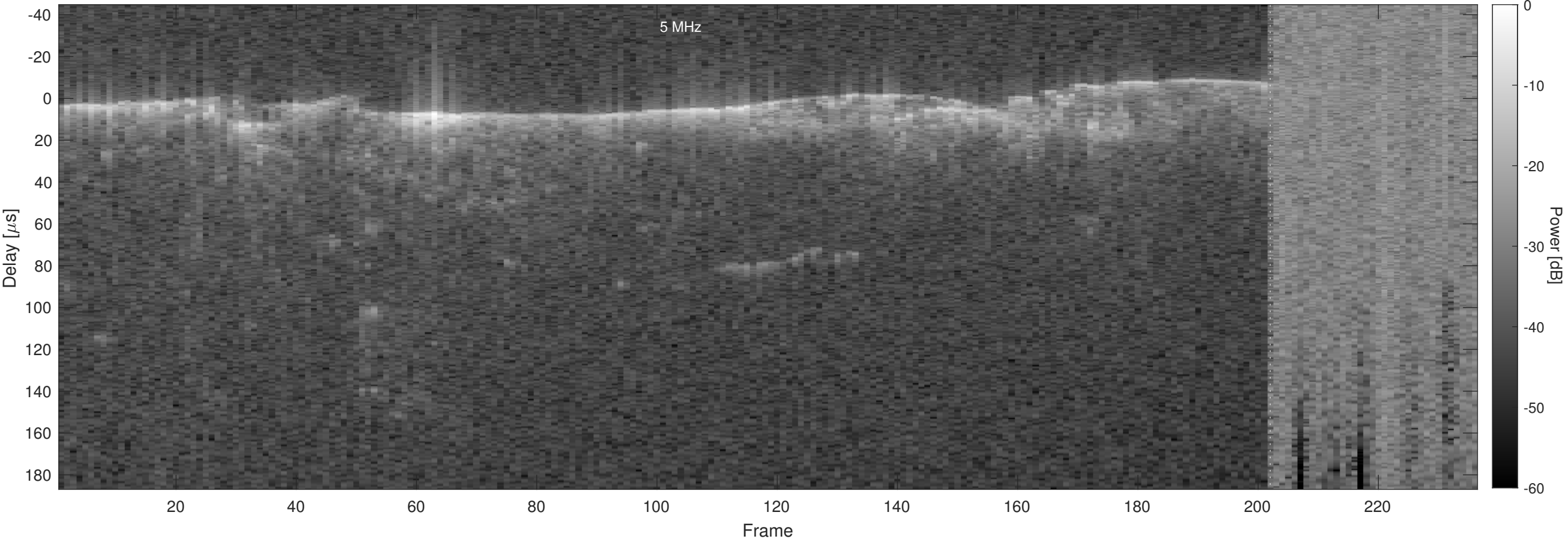
Orbit 2384, Optimized, No Window, Channel 2
