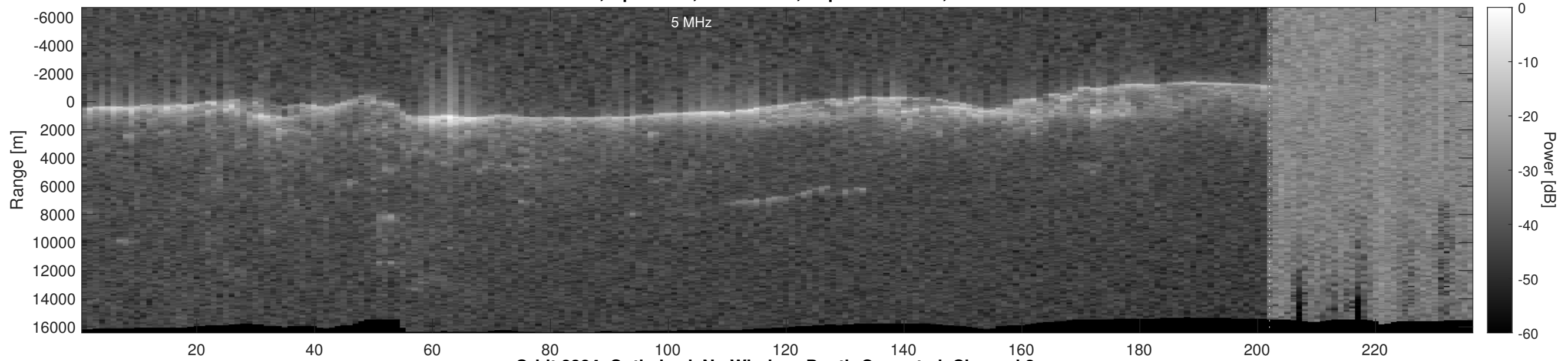
Orbit 2384, Optimized, No Window, Depth-Corrected, Channel 2
