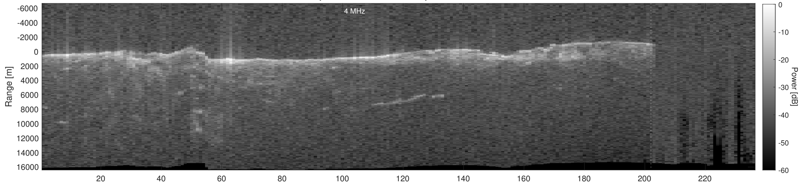
Orbit 2384, Depth-Corrected Cluttergram
