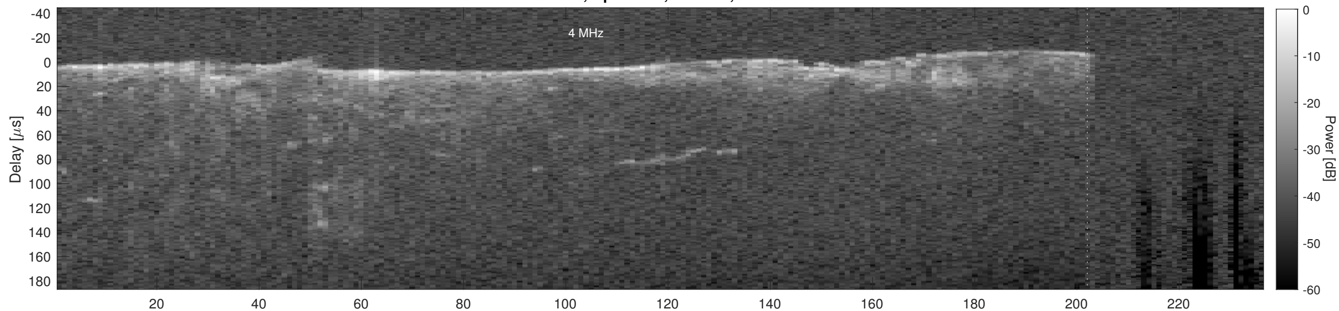
Orbit 2384, Cluttergram
