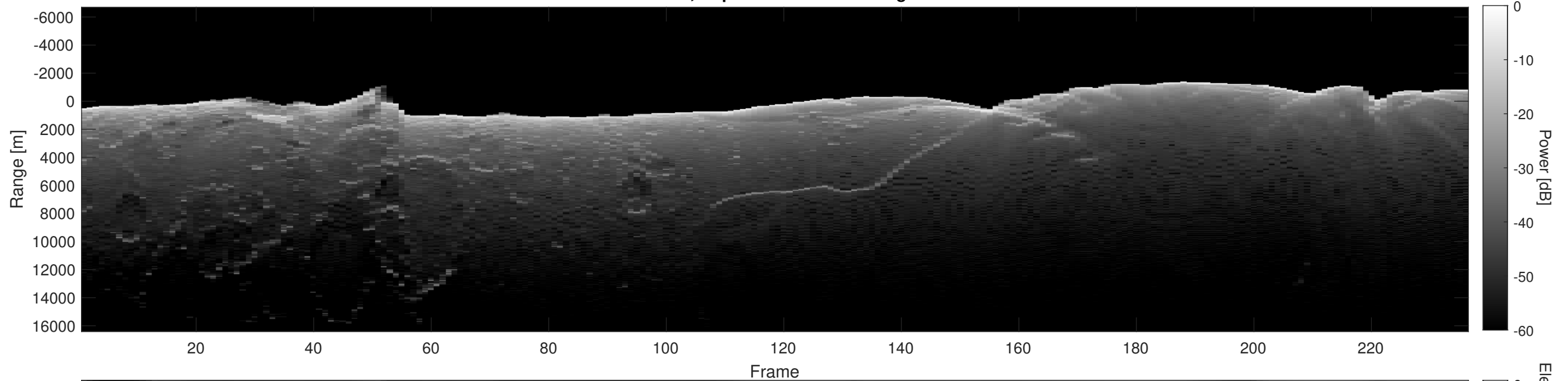
Orbit 2384, Depth-Corrected Cluttergram
