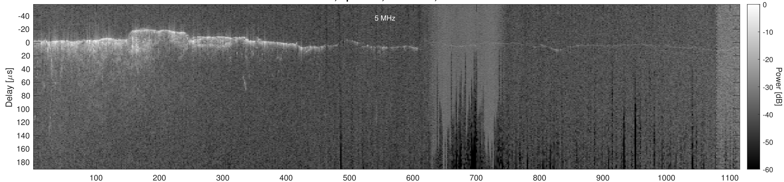
Orbit 2385, Optimized, No Window, Channel 2
