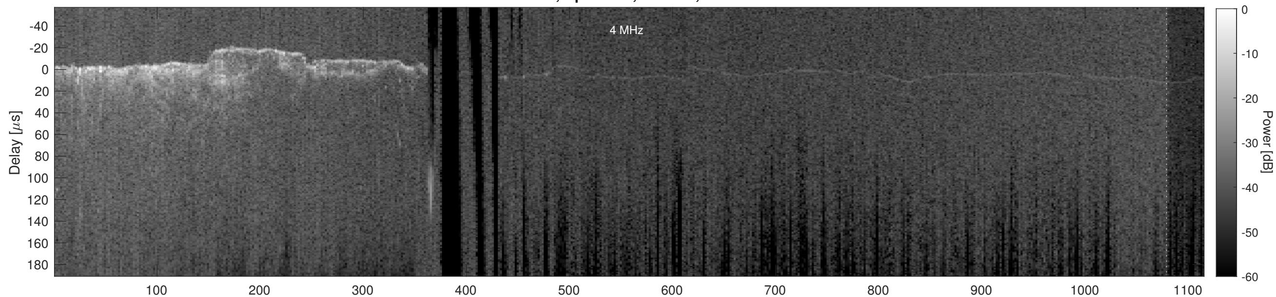
Orbit 2385, Cluttergram
