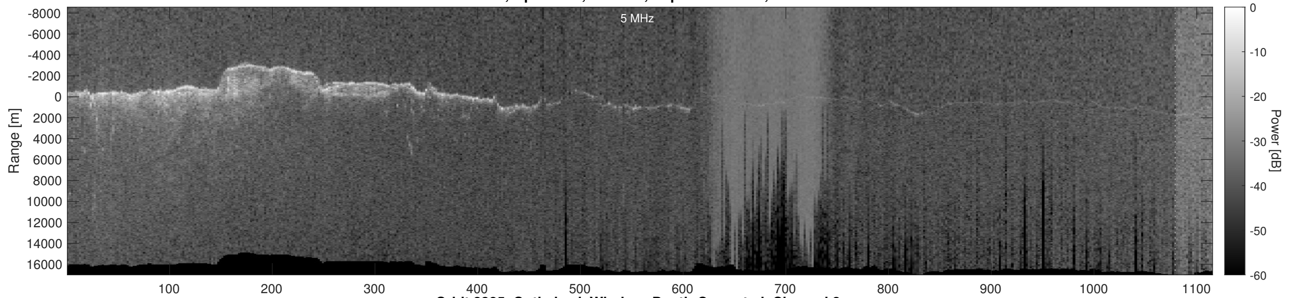
Orbit 2385, Optimized, Window, Depth-Corrected, Channel 2
