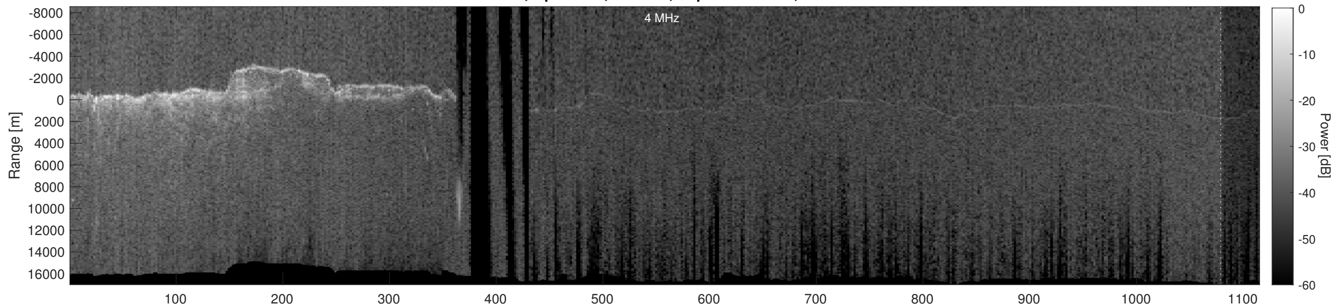
Orbit 2385, Depth-Corrected Cluttergram
