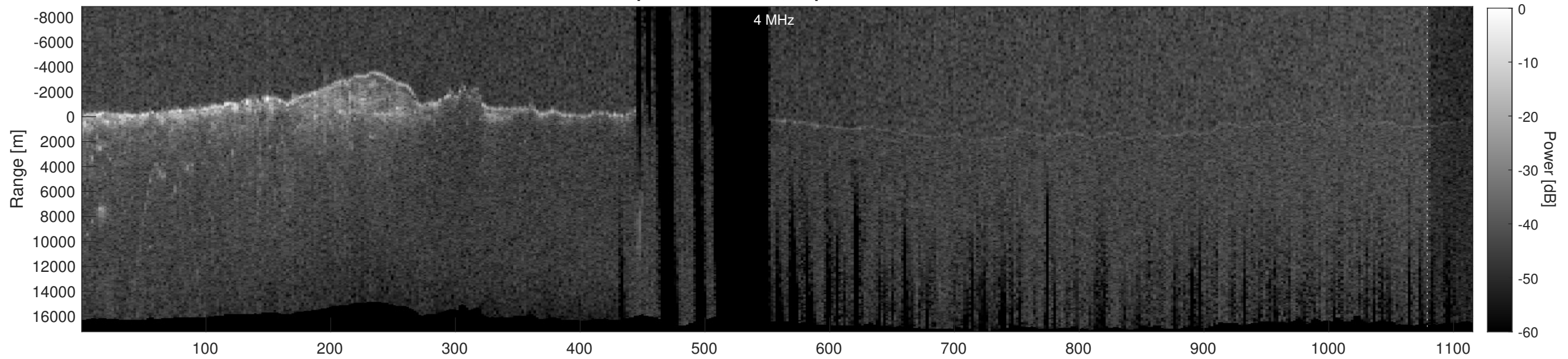
Orbit 2386, Depth-Corrected Cluttergram
