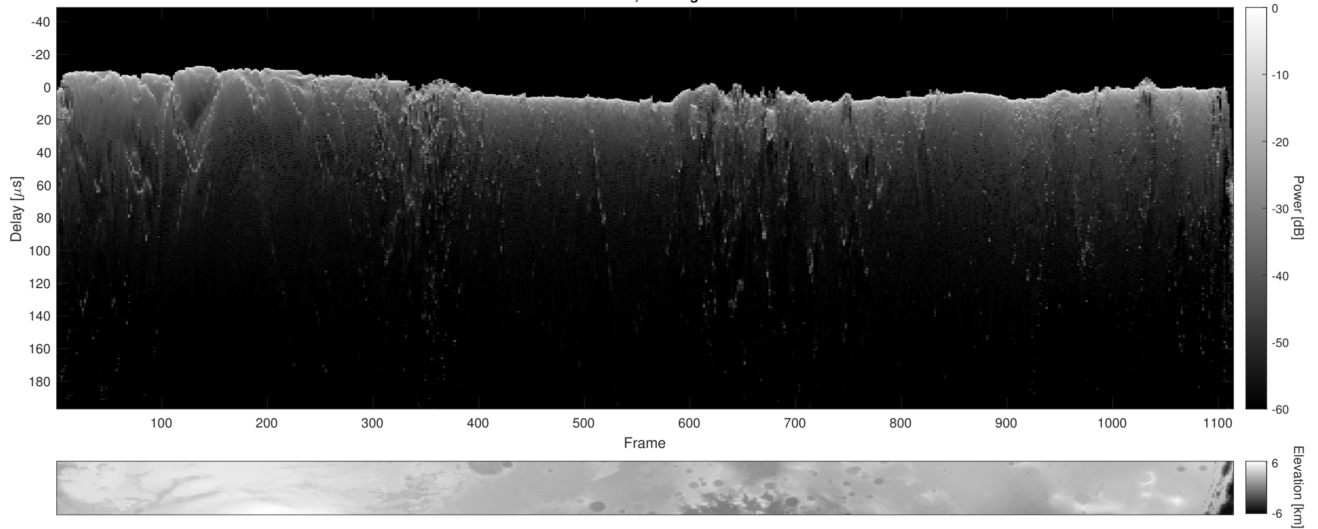
Orbit 2387, Cluttergram
