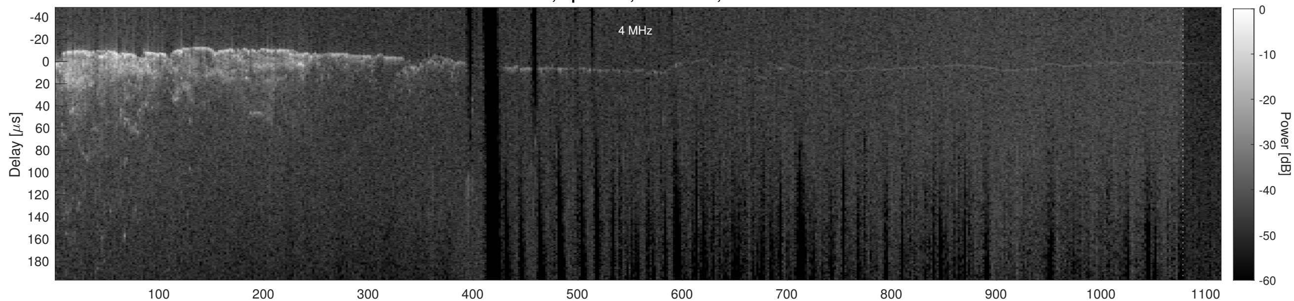
Orbit 2387, Cluttergram
