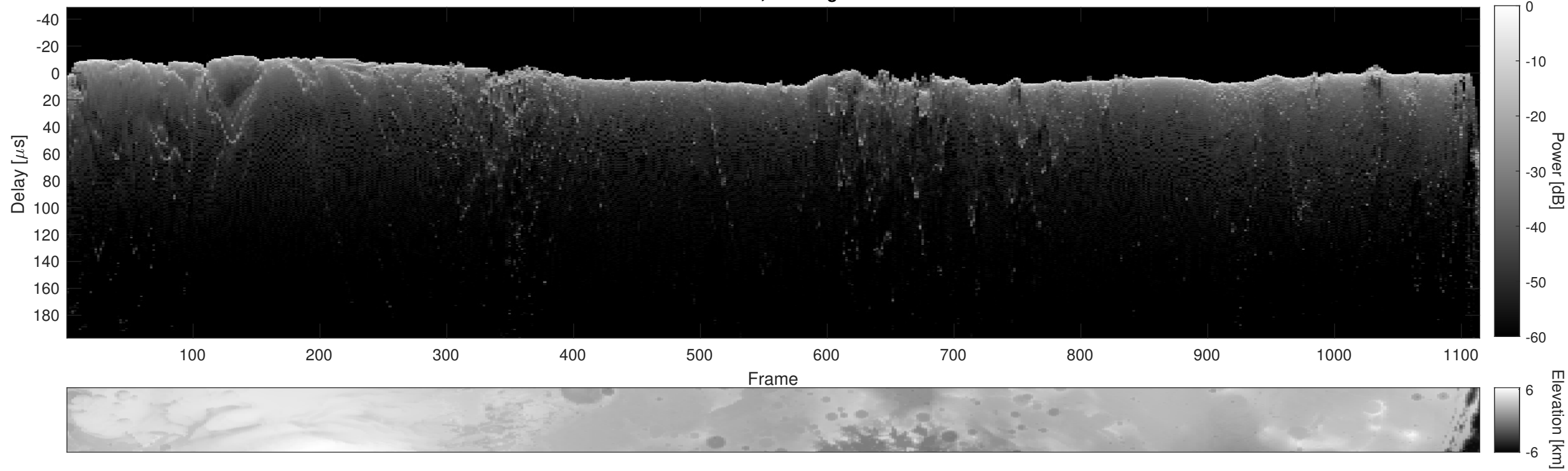
Orbit 2387, Cluttergram
