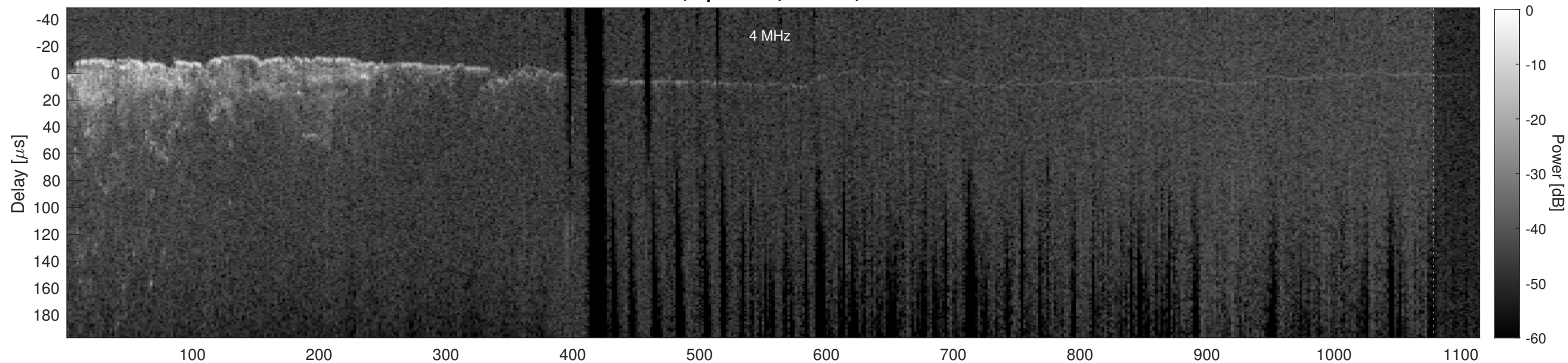
Orbit 2387, Cluttergram
