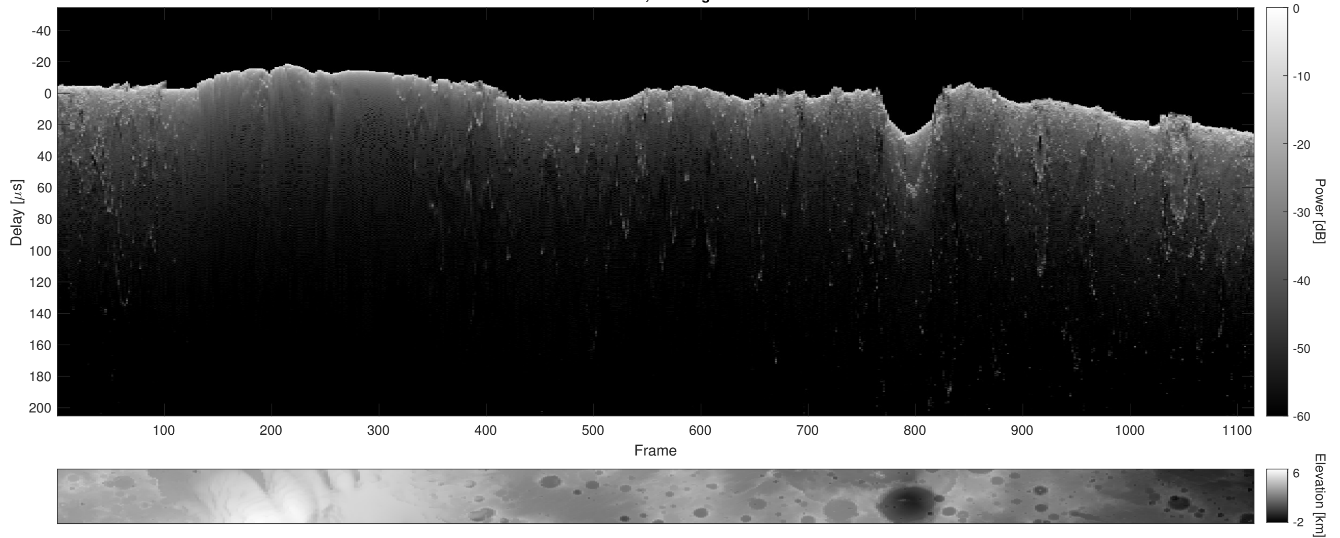
Orbit 2388, Cluttergram
