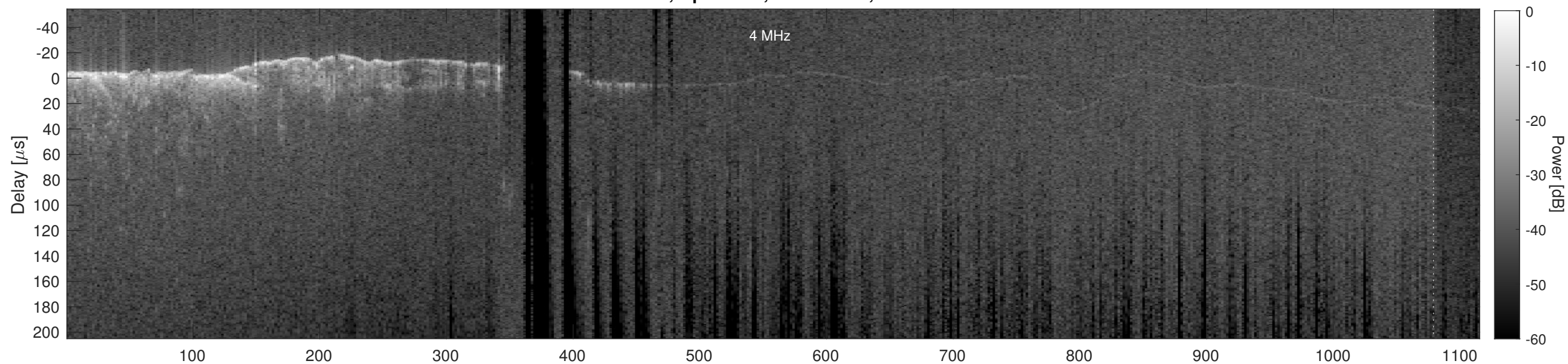
Orbit 2388, Cluttergram
