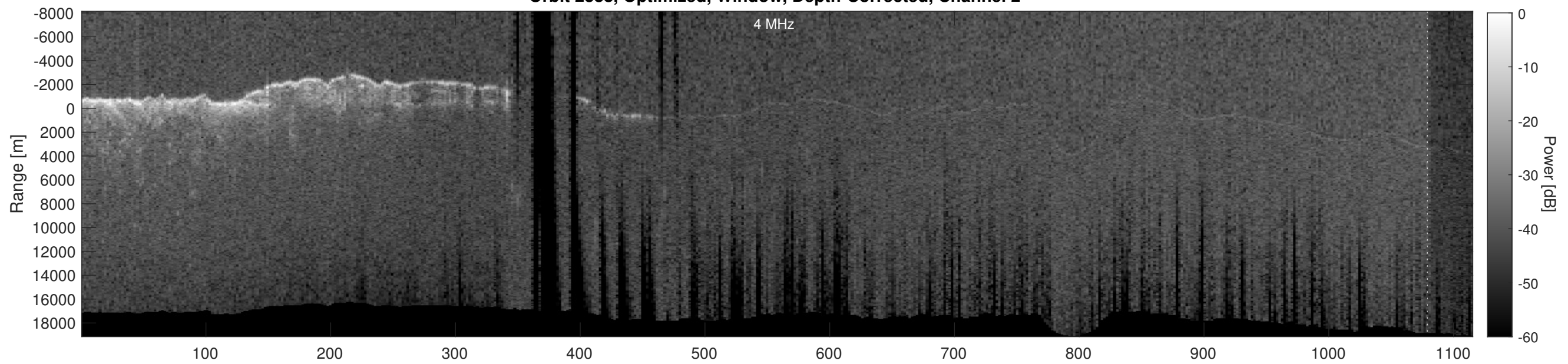
Orbit 2388, Depth-Corrected Cluttergram
