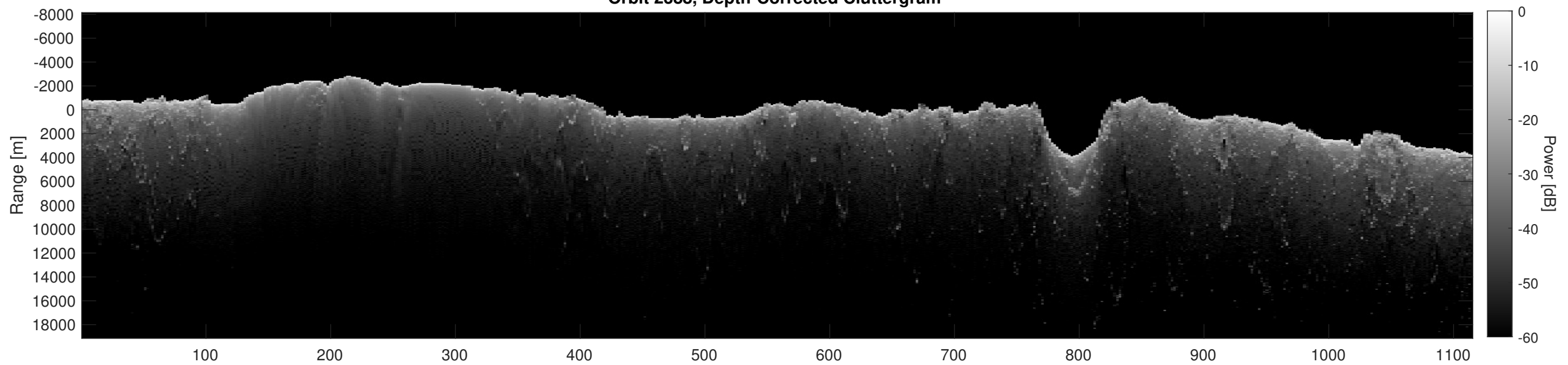
Orbit 2388, Depth-Corrected Cluttergram
