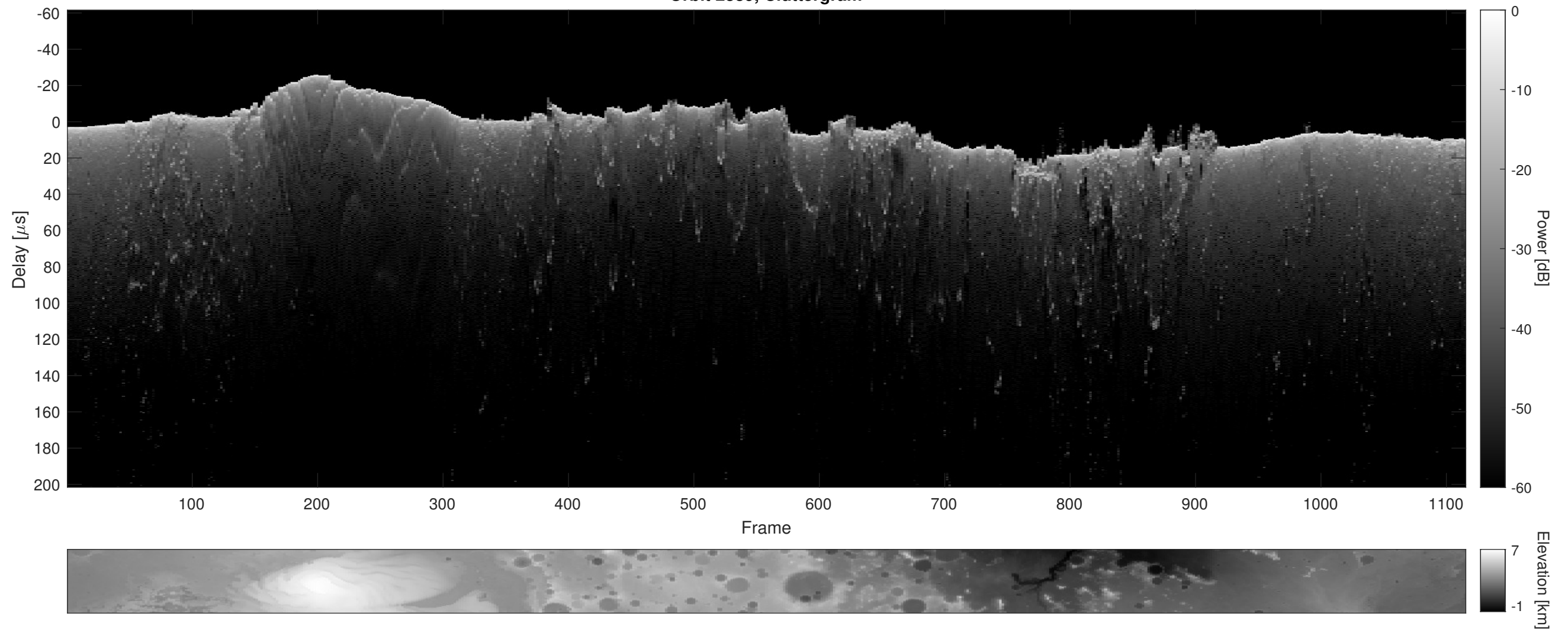
Orbit 2389, Cluttergram
