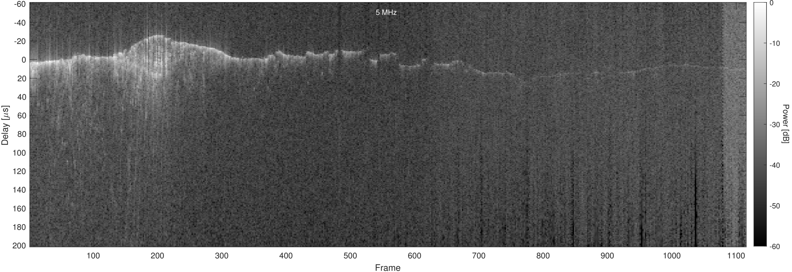
Orbit 2389, Optimized, No Window, Channel 2
