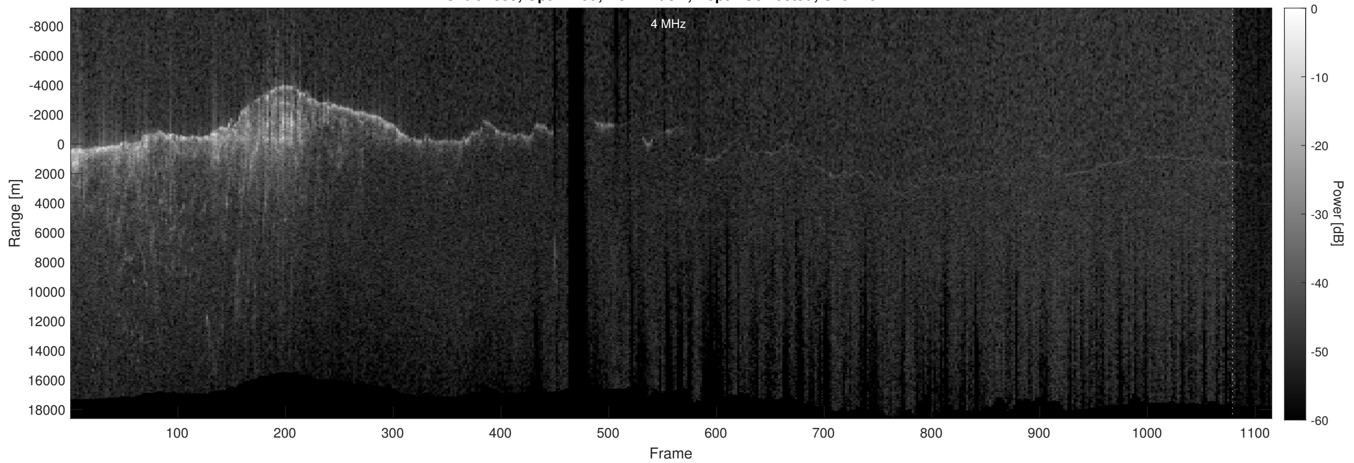
Orbit 2389, Optimized, No Window, Depth-Corrected, Channel 2
