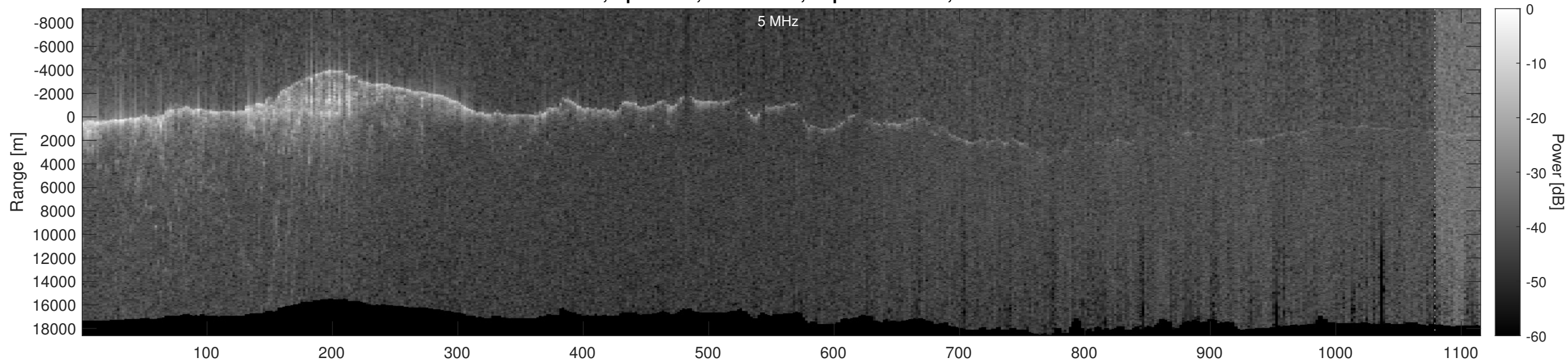
Orbit 2389, Optimized, No Window, Depth-Corrected, Channel 2
