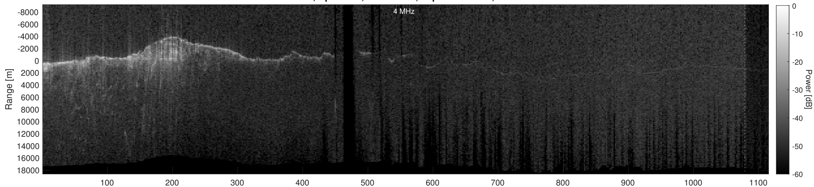
Orbit 2389, Depth-Corrected Cluttergram
