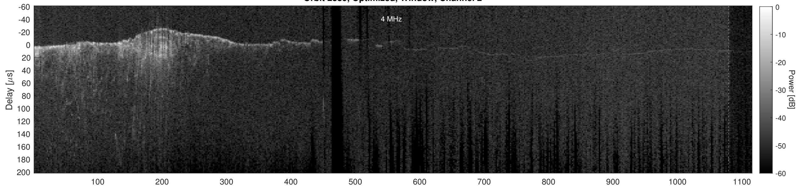
Orbit 2389, Cluttergram
