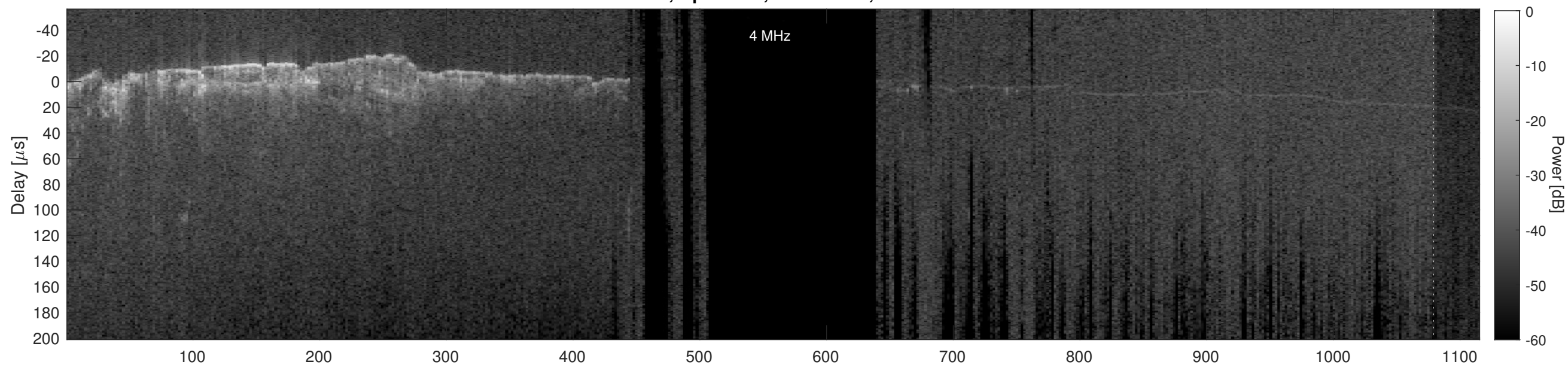
Orbit 2390, Cluttergram
