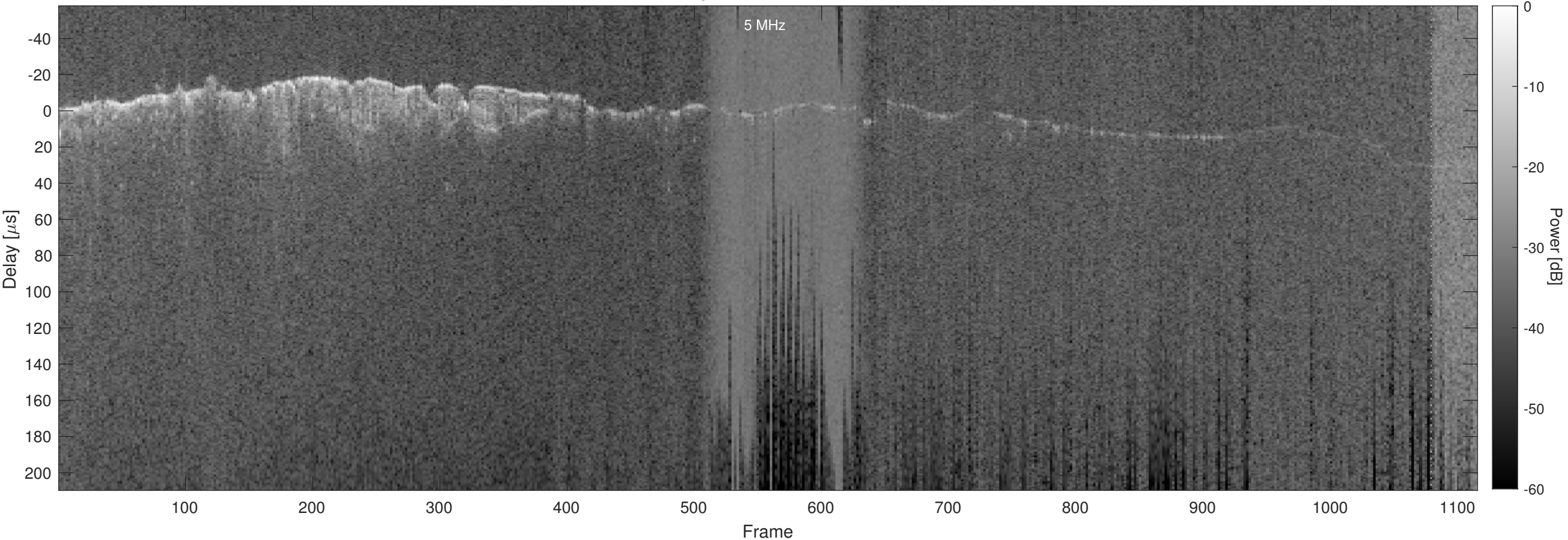
Orbit 2392, Optimized, Window, Channel 2
