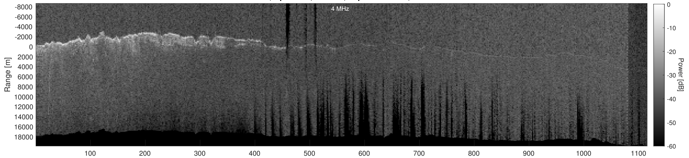
Orbit 2392, Depth-Corrected Cluttergram
