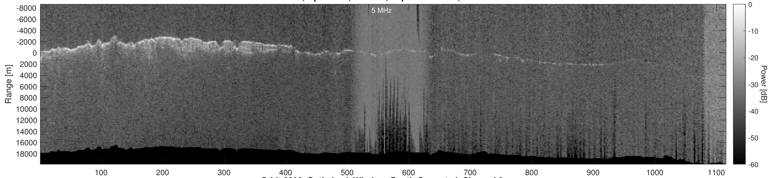
Orbit 2392, Optimized, Window, Depth-Corrected, Channel 2
