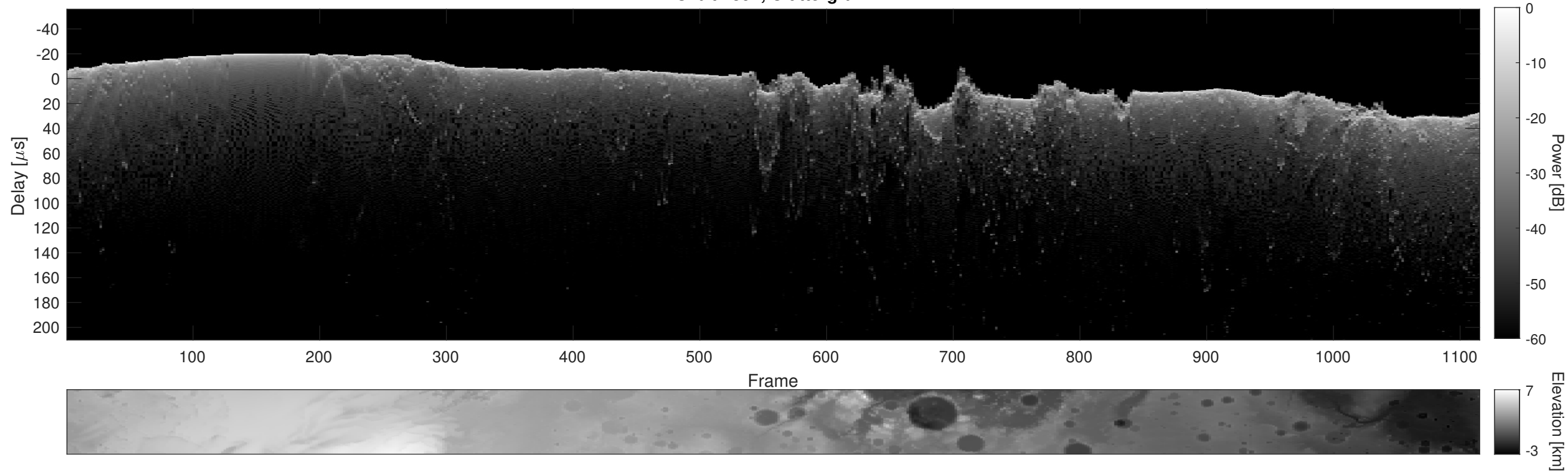
Orbit 2394, Cluttergram
