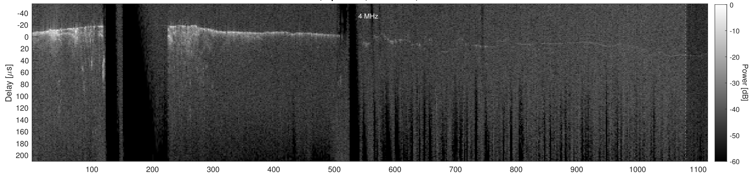
Orbit 2394, Cluttergram
