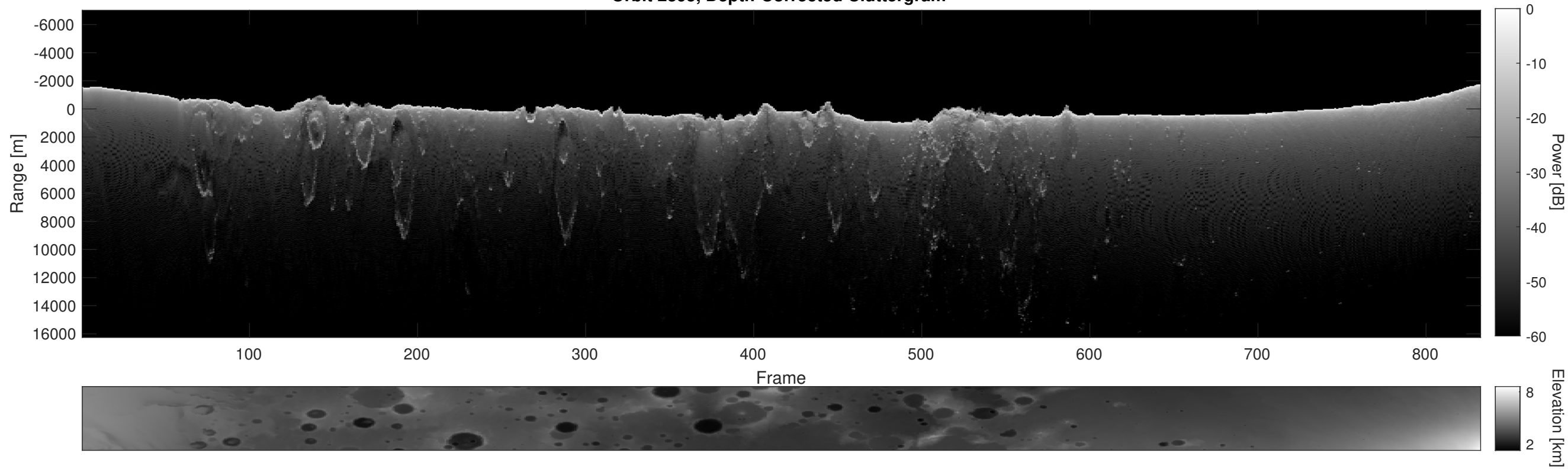
Orbit 2395, Depth-Corrected Cluttergram
