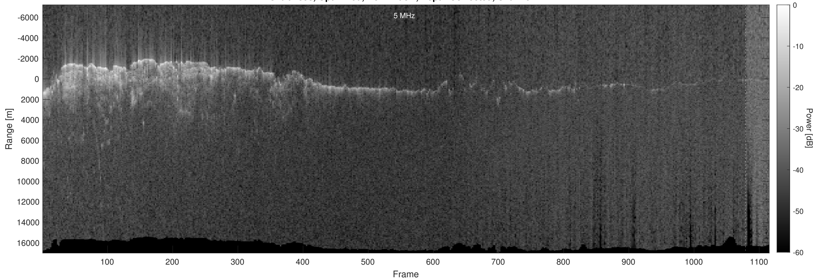
Orbit 2398, Optimized, No Window, Depth-Corrected, Channel 2
