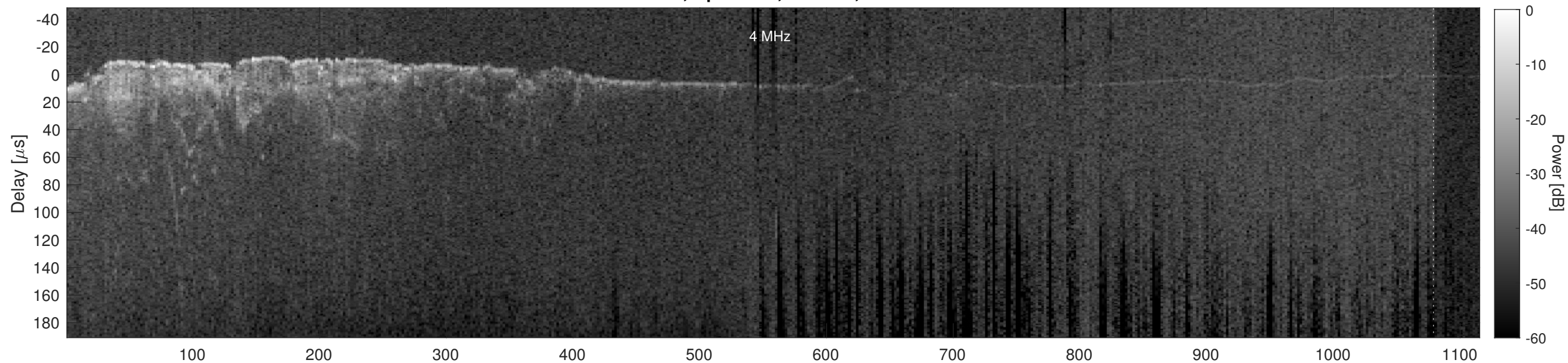
Orbit 2398, Cluttergram
