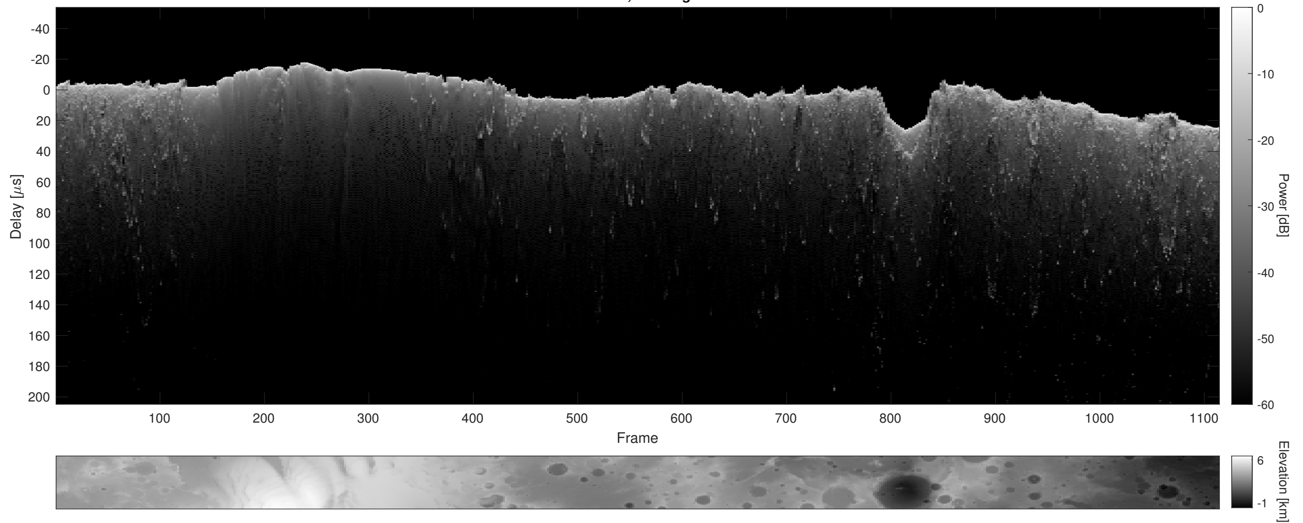
Orbit 2399, Cluttergram
