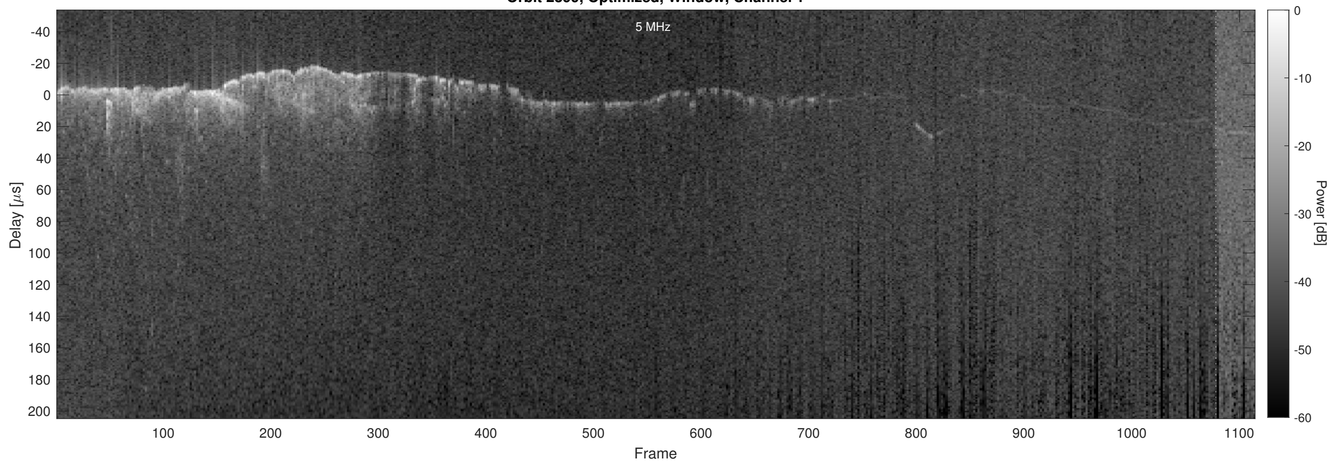
Orbit 2399, Optimized, Window, Channel 2
