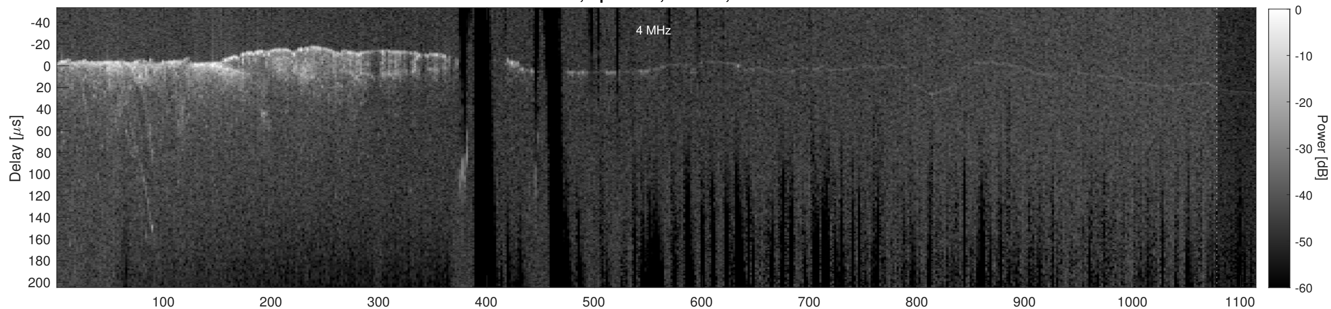
Orbit 2399, Cluttergram
