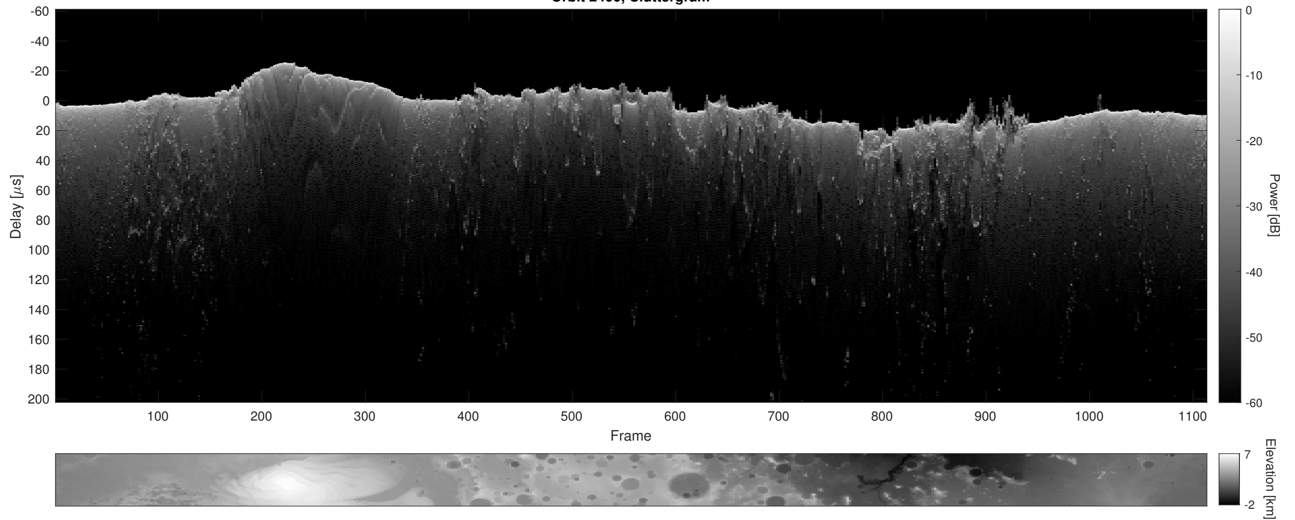
Orbit 2400, Cluttergram
