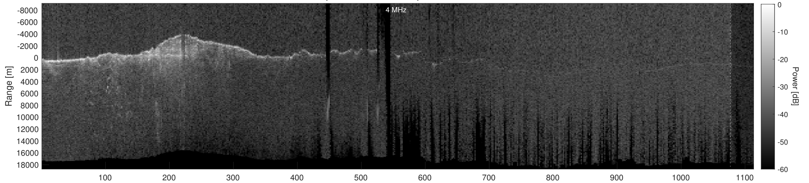
Orbit 2400, Depth-Corrected Cluttergram
