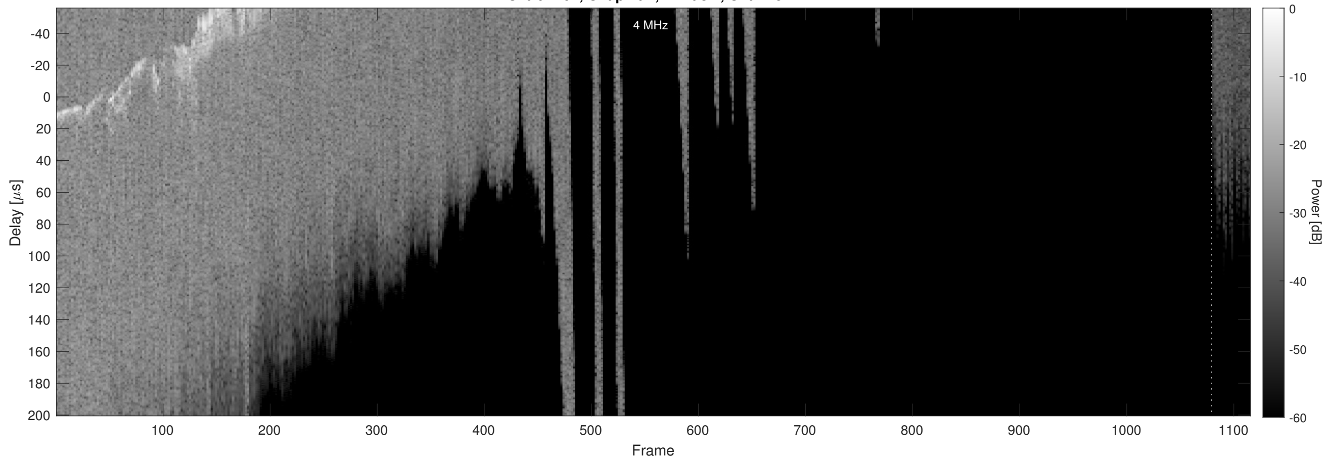
Orbit 2401, Chapman, Window, Channel 2
