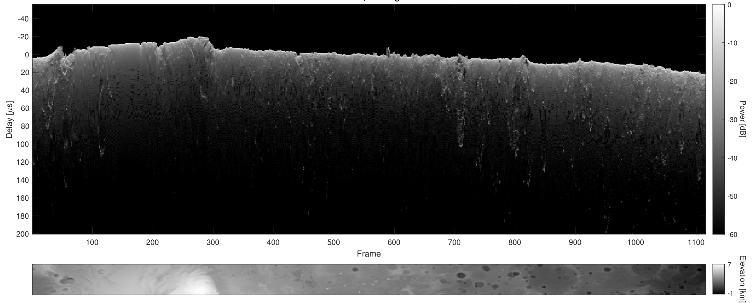
Orbit 2401, Cluttergram
