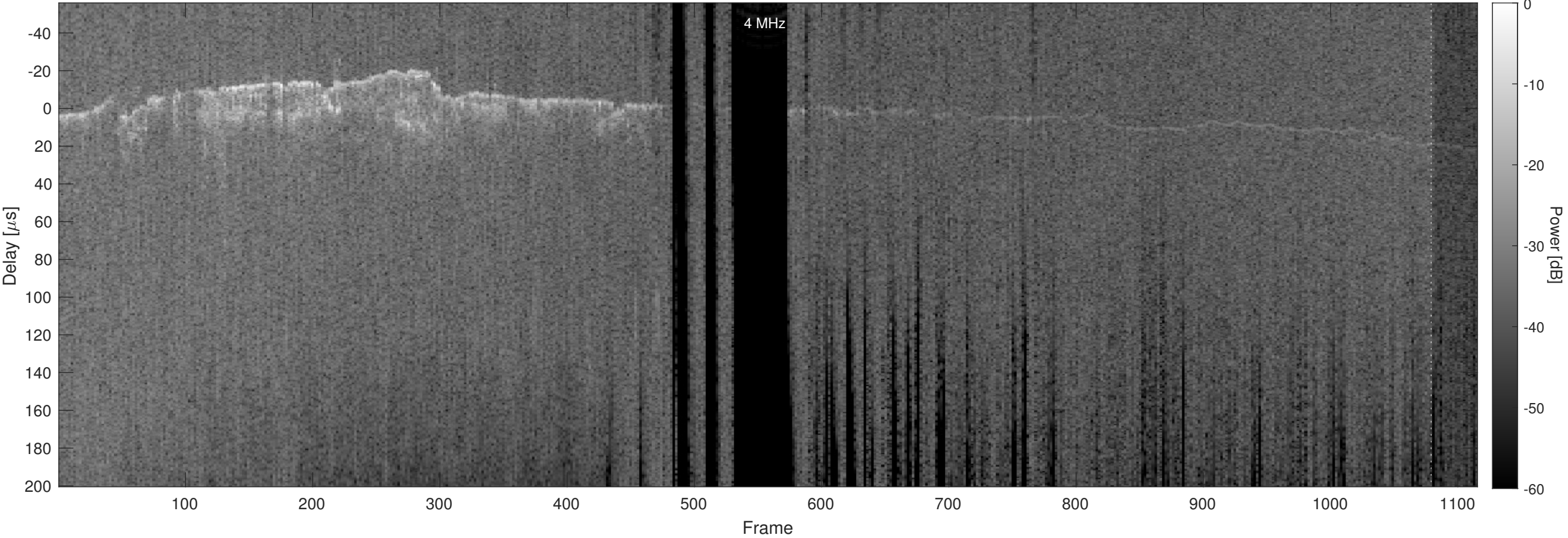
Orbit 2401, Optimized, No Window, Channel 2
