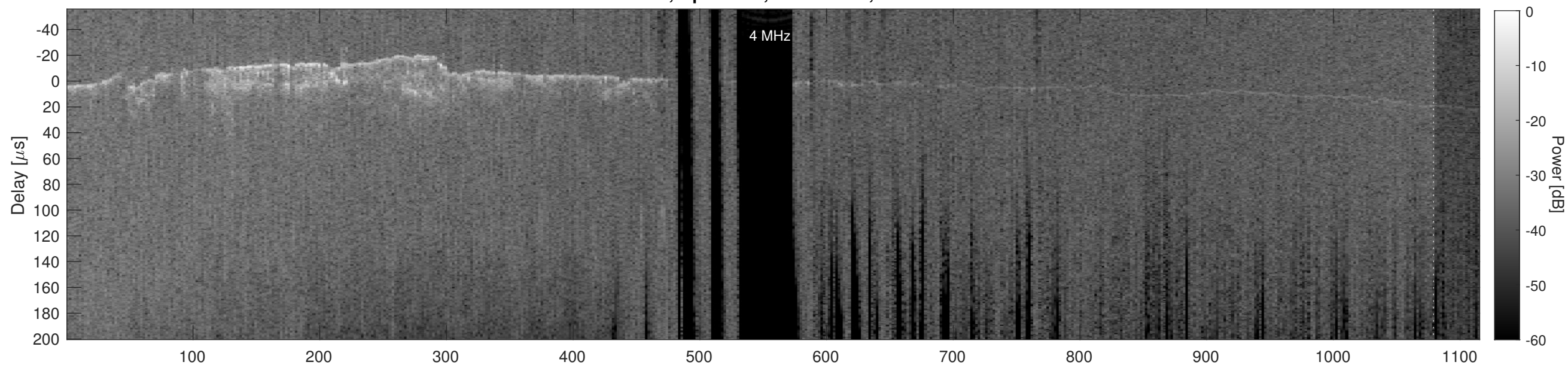
Orbit 2401, Cluttergram
