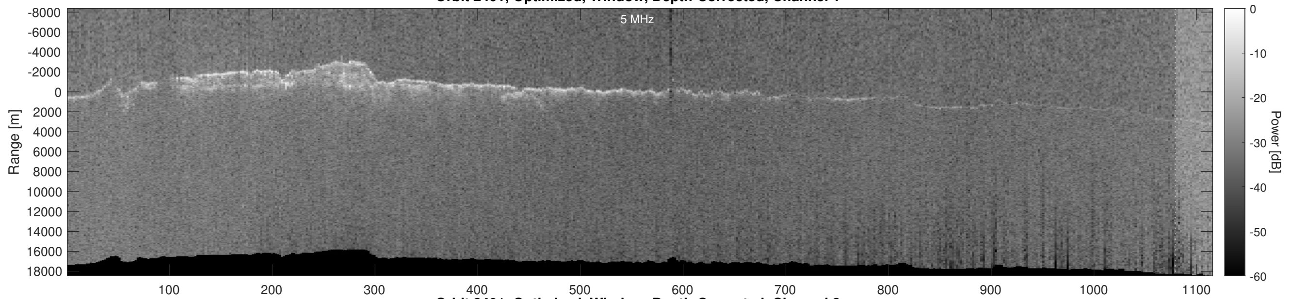
Orbit 2401, Optimized, Window, Depth-Corrected, Channel 2
