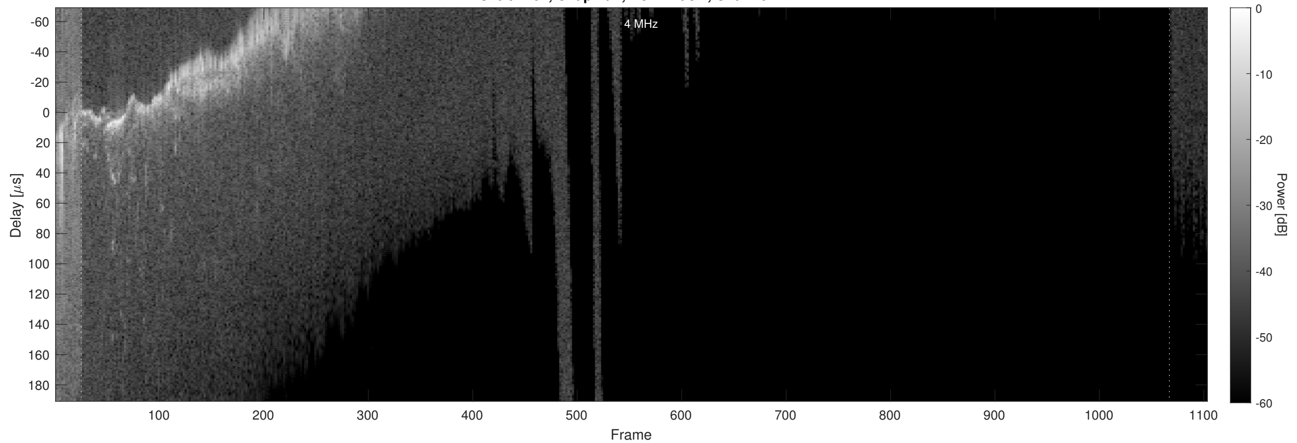
Orbit 2402, Chapman, No Window, Channel 2
