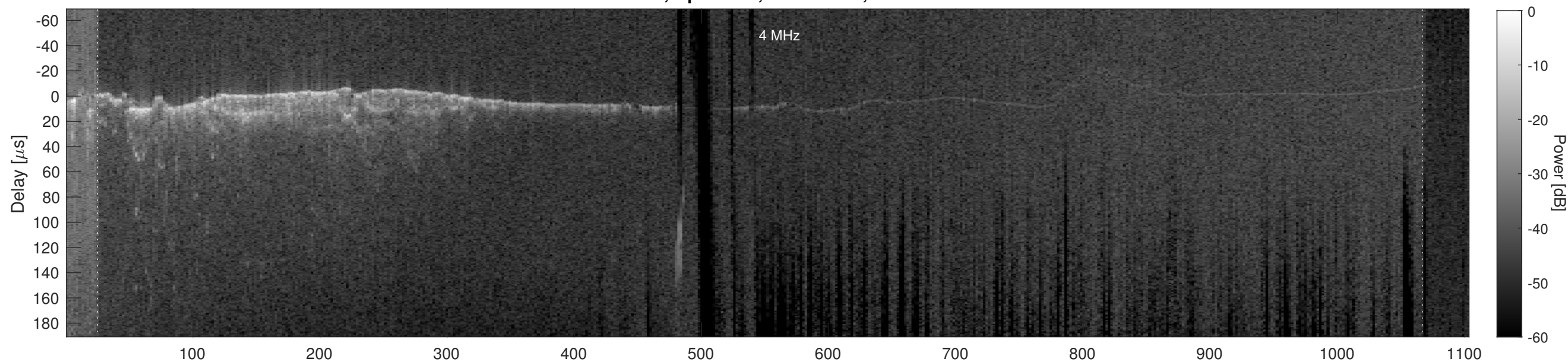
Orbit 2402, Cluttergram
