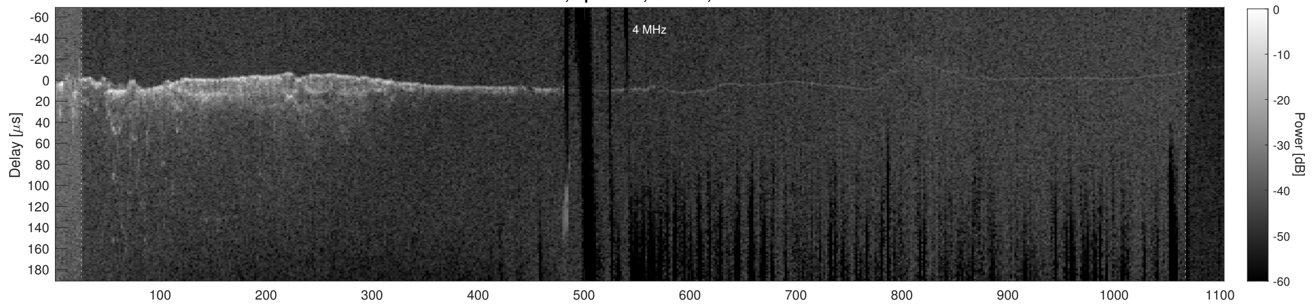
Orbit 2402, Cluttergram
