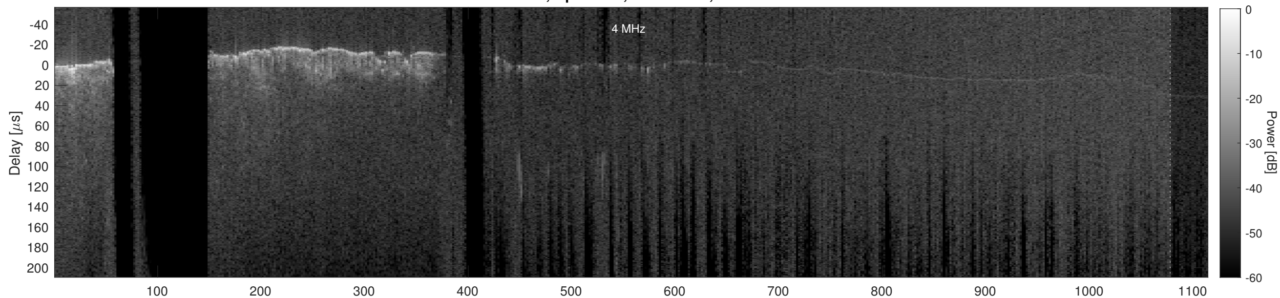
Orbit 2403, Cluttergram
